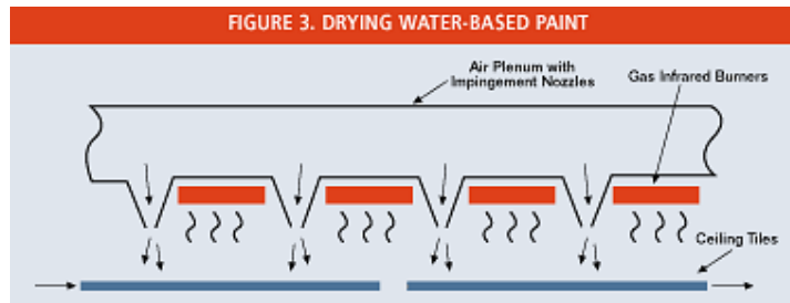
Combination convection/infrared commonly is used for drying water-based coating on ceiling tiles. Convection helps speed drying by removing the microscopic layer of moist, saturated air that forms on the surface.
